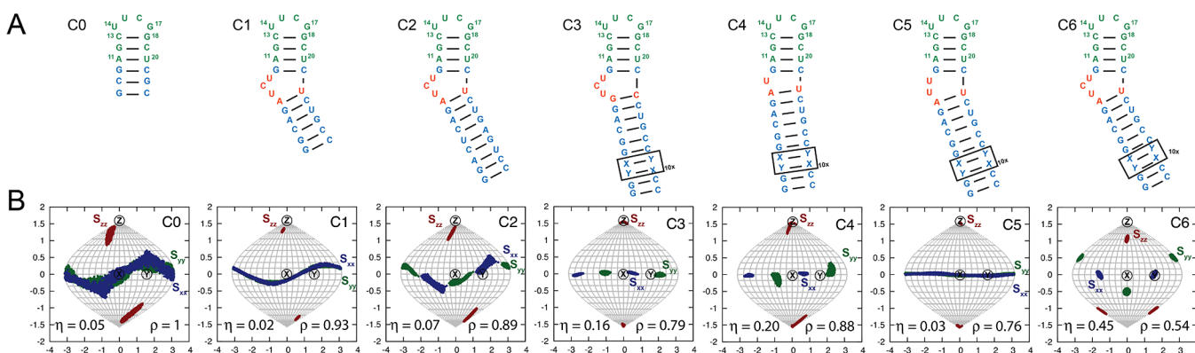
Figure 1. Kinked elongated constructs of cUUCGg apical loop. (A) The alignment of the studied motif (green) is modulated by the kinked elongated strategy: helical parts (blue), bulge (orange). The constructs are labeled from C0 to C6. (B) Sauson–Flamsteed projection maps depicting the order tensor frame ( S_{zz} , S_{yy} , S_{xx} ) relative to a frame of reference in which the helix axis of the upper helix are aligned parallel to the molecular z direction. Also shown is the asymmetry of alignment ( \eta = |S_{yy} - S_{xx}|/S_{zz} ) and \rho values which represents the scalar product of the alignment tensor for a given construct with that of C0 (see Methods).
