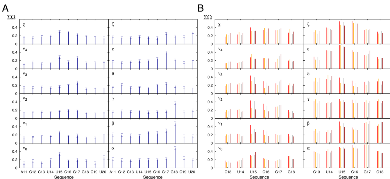
Figure 4. Conformational variability in the MD-derived and RDC-selected ensemble of the cUUCGg hairpin. (A) Shown is the \Sigma\Omega value between the MD and RDC-selected ensemble for all the backbone and sugar dihedral angles. A decrease in \Sigma\Omega indicates an increase in similarity. Error bars are derived from Monte Carlo simulations (Methods). (B) \Sigma\Omega value comparing the structural pool of the cUUCGg loop from the PDB (Methods) and the RDC-selected ensemble (red) or the MD trajectory (gray). Shown in orange and brown is the corresponding comparison when restricting the PDB structures to unbound RNA.
