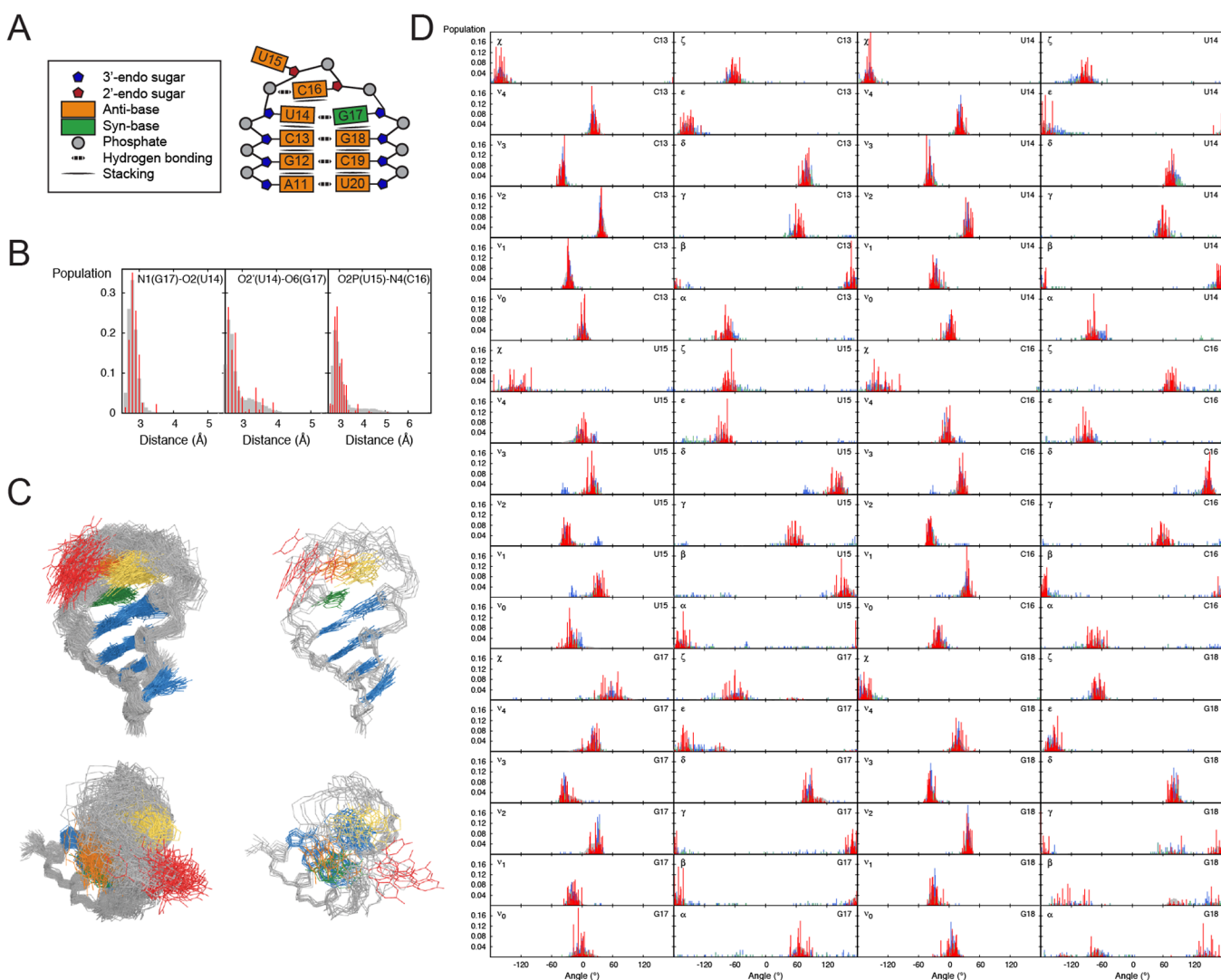
Figure 3. Comparison of the MD and RDC-selected ensembles for the cUUCG tetraloop. (A) Schematic representation of the interactions and structural features of the cUUCG loop. (B) Distance distributions between N1(G17)-O2(U14), O2'(U14)-O6(G17), and O2P(U15)-N4(C16) that describe the H-bonding interaction between U14-G17 and U15-C16 in the MD (gray) and the RDC-selected ensemble (red) (C) Comparison of 100 randomly selected conformers from the MD (left) and RDC-selected ensemble (right), coordinates are included in the Supporting Information . (D) Comparison of dihedral angle distributions in the cUUCG loop from the MD (gray), RDC-selected ensembles (red), and ensemble representing the cUUCG structures in the PDB with (blue) and without (green) bound proteins and ligands.
