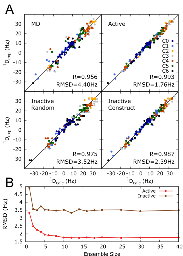
Figure 2. Constructing a cUUCGg tetraloop ensemble using RDCs derived from kinked elongation and an MD simulation. (A) Agreement between measured RDCs color coded for different kinked elongated constructs and values back predicted using the MD-generated (0.8 \mu s MD simulation using the AMBER ff10 force field) and RDC-selected ensemble with N = 10 conformers (Active). Also shown is the cross-validated agreement between measured RDCs and RDCs that was left out from the sample and select analysis when randomly omitting \sim 13\% of the data (Inactive Random) or entire RDC data set for an individual kinked elongated construct (Inactive Construct). Shown in each case is the RMSD and Pearson's correlation coefficient. (B) RMSD between measured and back-predicted RDCs as a function of number of conformers used in the sample and select analysis to construct ensemble. Values are shown when including all RDCs in the selection (active) and for RDCs randomly left out of the selection (inactive).
