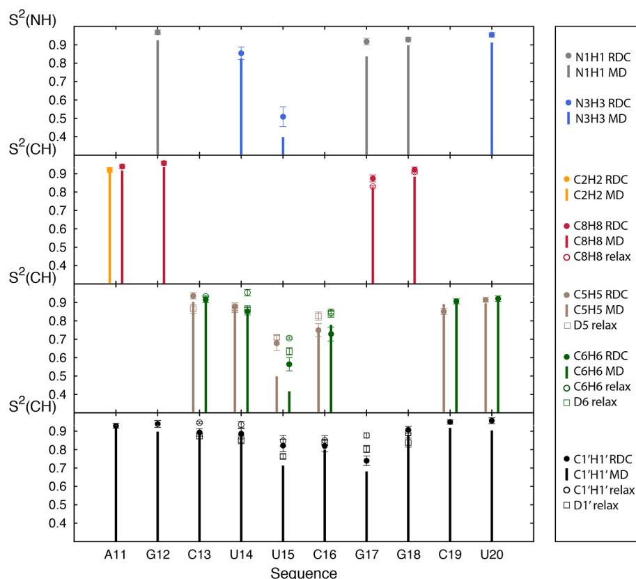
Figure 5. Conformational disorder in the cUUCGg tetraloop. Comparison of the order parameter ( S^2 ) of several bound vectors N1H1 (gray), N3H3 (blue), C2H2 (orange), C8H8 (red), C5H5 and D5 (brown), C6H6 and D6 (green), and C1'H1' and D1' (black). Bars correspond to the order parameters computed for the entire MD trajectory, filled circle to the order parameter computed for the RDC-selected ensemble, open circles to ^{13}\text{C} spin relaxation order parameter measured on a related cUUCGg tetraloop, 69 and open rectangles to ^2\text{H} spin relaxation order parameter measured on a related cUUCGg tetraloop. 70 The RNA sequence between the current and ^2\text{H} relaxation study matches only residues 13–18, and differences in sequence could affect order parameters especially for residues 13 and 18. Error bars for the RDC-selected ensemble are obtained using Monte Carlo simulations (see Methods ).
